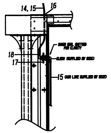
AIR LINE ROUTING DETAIL
