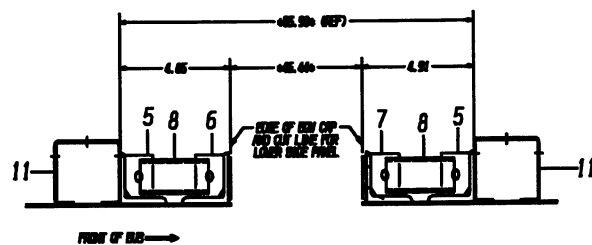
TOP VIEW SECTION THROUGH DOOR OPENING
