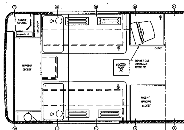
Twin Bed Option
