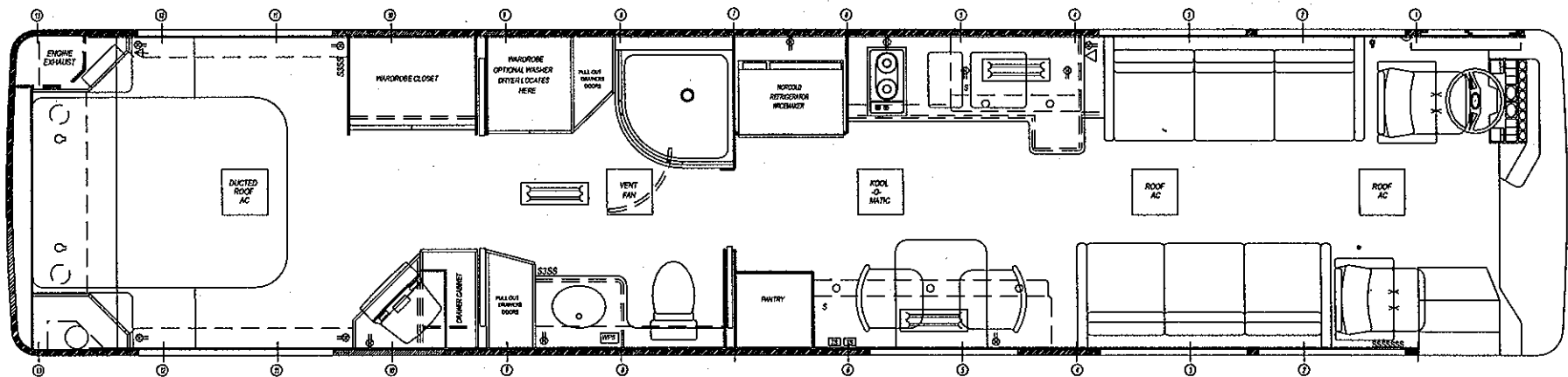
1999 Wanderlodge LX Floorplan "D" shown with standard center island bed
