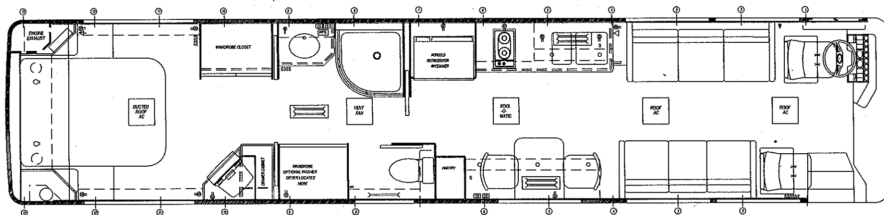
1999 Wanderlodge LX Floorplan "C"
