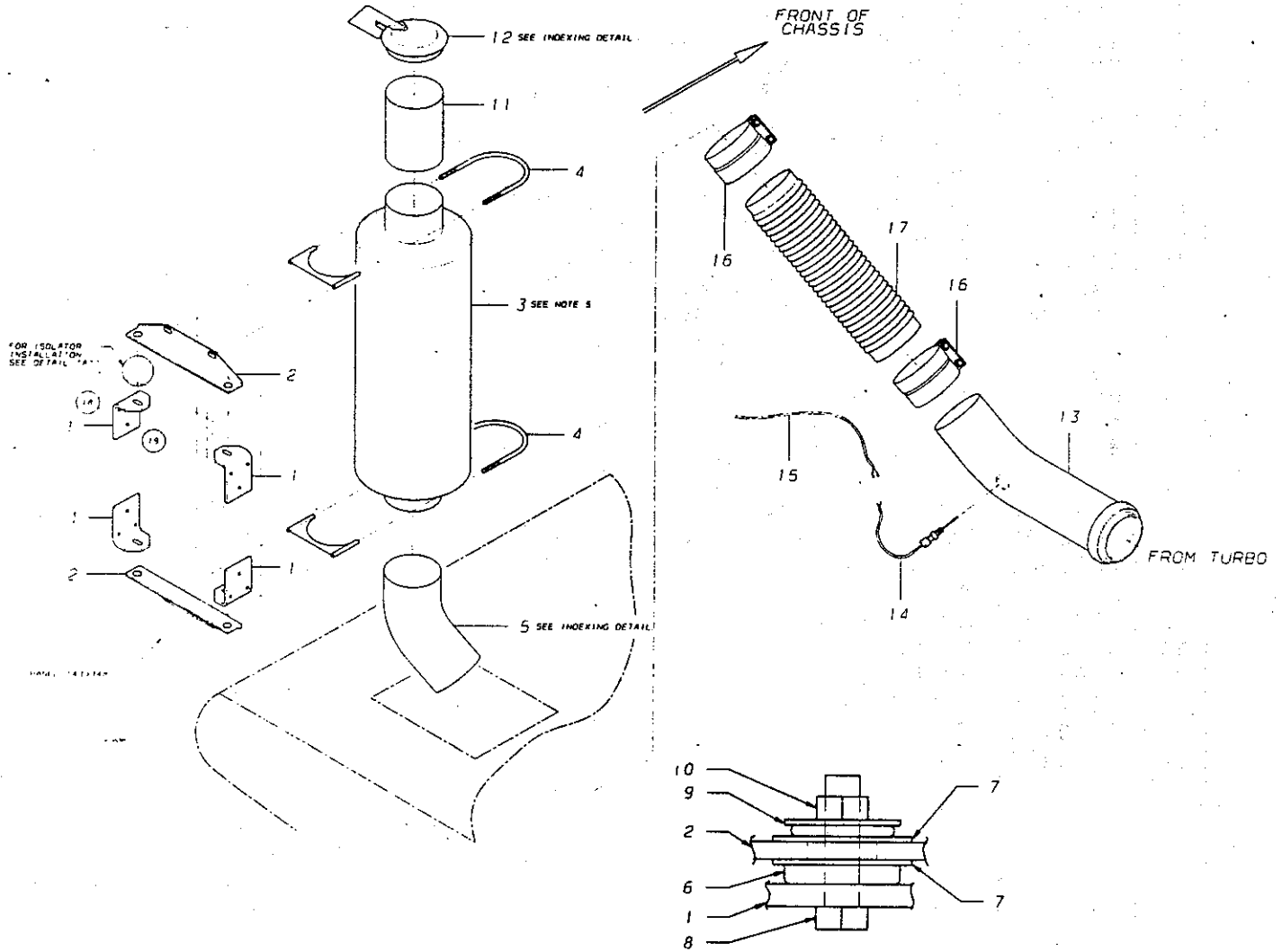
DETAIL 'A' (TYP. 4 PLACES)
