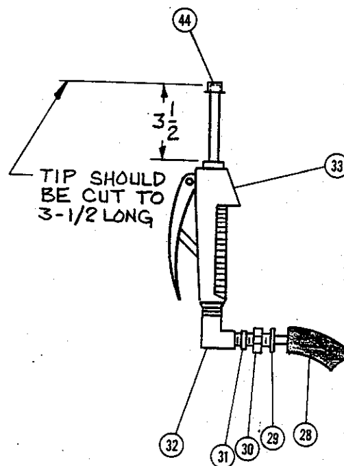
OIL CONTROL VALVE
