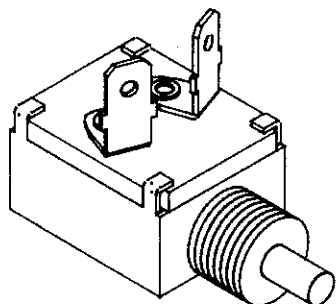
1126184 Switch, Momentary, 2 Terminals (Off When Out)
