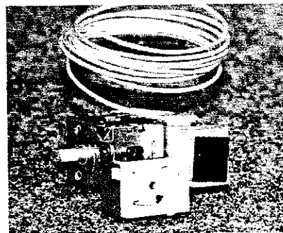
4401238 Thermostat, Refrigerator 1300
