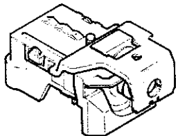
0952465 Switch, Headlight (8 Blade Type Terminals) 3839040 Switch, Headlight (6 Blade Type Terminals)
