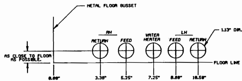
DETAIL "A" 1/2 SCALE
