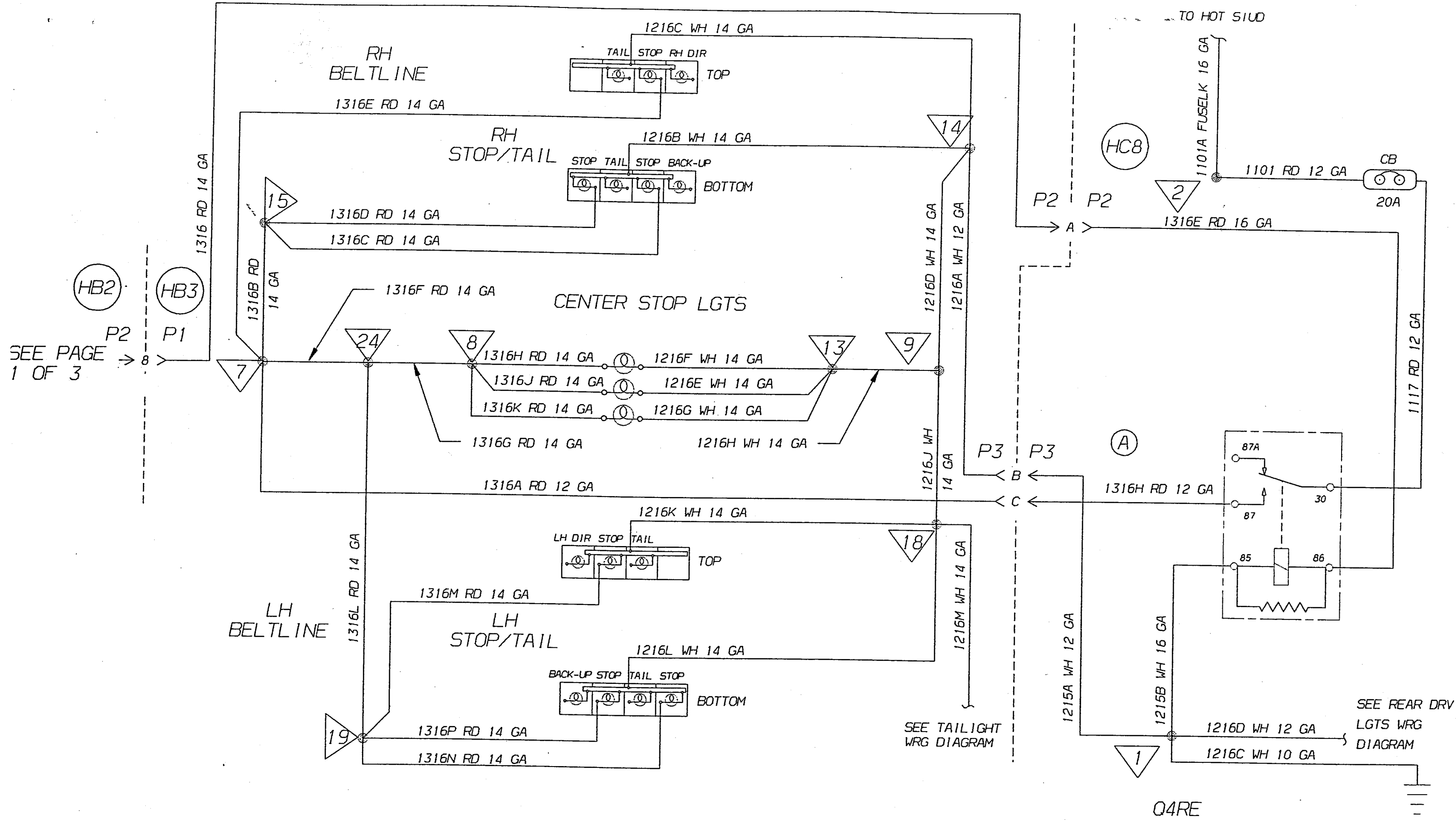
D. WRG. STOP LIGHTS DDEC 0010397 #2M
