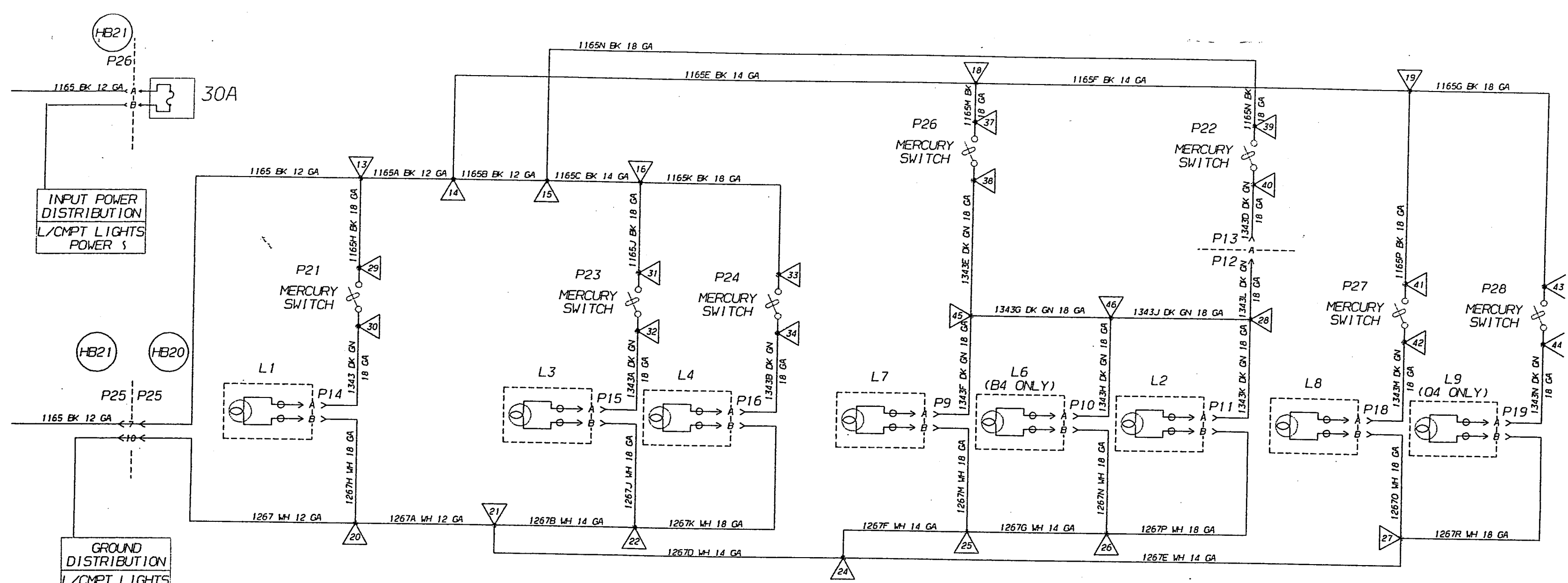
LIGHT ASSEMBLY IDENTIFICATION DIAGRAM
