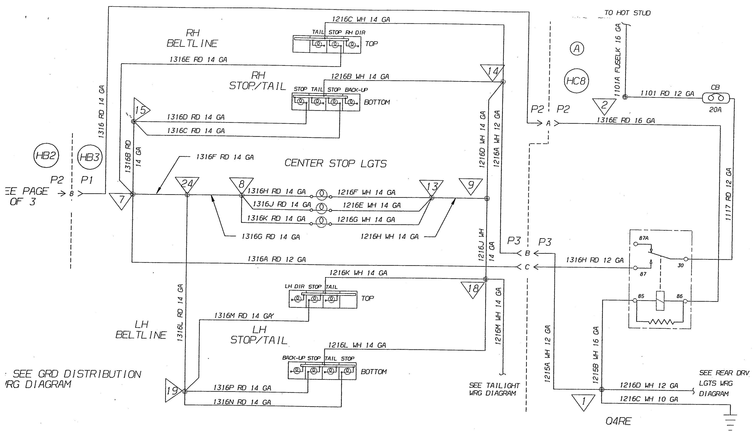
D. WRG. STOP LIGHTS M11 0010405 #2
