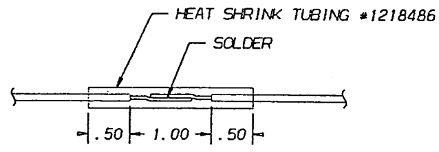
SPLICE DETAIL.
