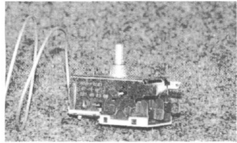
3783974 Thermostat, Refrigerator 1303
