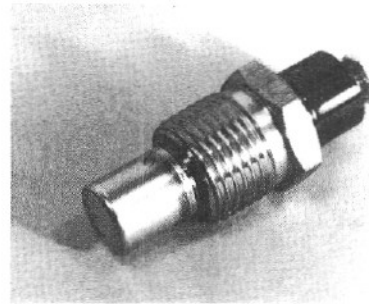
4176483 Switch, High Water Temperature Shut-Down (Perkins Generator)
