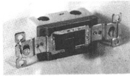
2224434 Switch, Engine Block - 3 Terminals (15A, 120/277 VAC)
