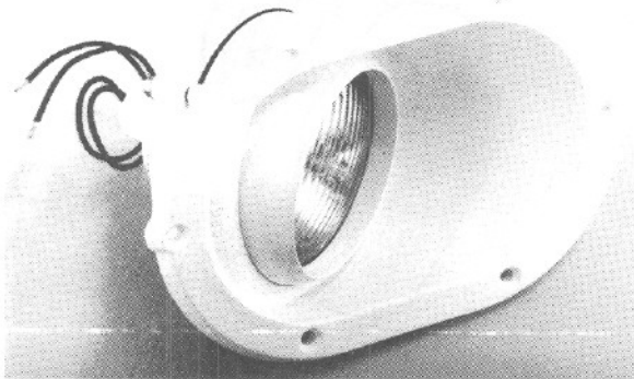
2223733 Light Assembly, Landing/Docking 2261626 Bulb, Sealed Beam
