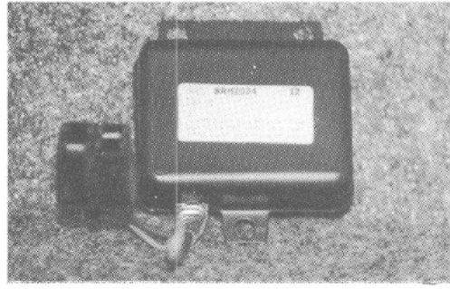
0882167 Regulator, Alternator
