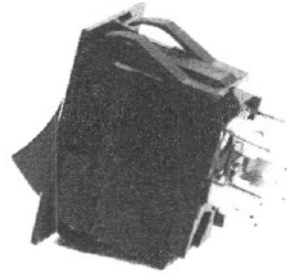
3887023 Switch, Pilot/Co-Pilot Seat (4 Terminals-20 AMP-250 VAC)
