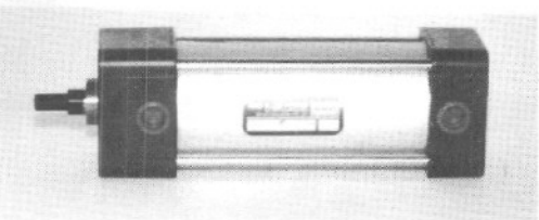
2273043 Cylinder, Air, 2 1/2" Bore X 4 1/2" Stroke Aro. No. 1825-1009-1-044 Entrance Door Steop WLFC, WLPP 1981-85
