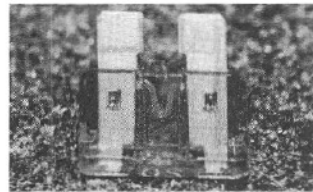
3866761 Fuse, Plug In Type, 30 Amp 3866738 Fuse, Plug In Type, 20 Amp 3866712 Fuse, Plug In Type, 10 Amp 3866720 Fuse, Plug In Type, 15 Amp 3866753 Fuse, Plug In Type, 5 Amp 3866746 Fuse, Plug In Type, 3 Amp
