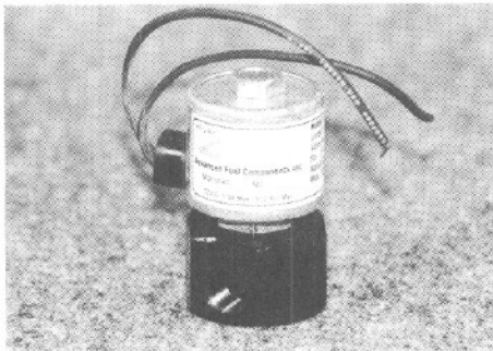
3940897 Solenoid, LPG Upright
