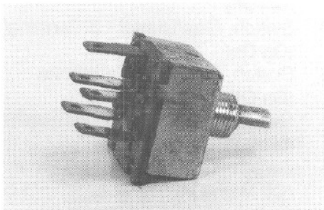
3856721 Switch, Chassis Air Dash (25 Amp - 5 Terminals)
