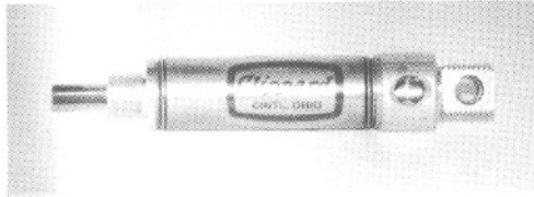
3797875 Cylinder, Air, 3/4" Bore 1" Stroke, Pilot Fresh Air
