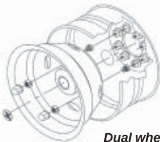
Dual wheel rear
